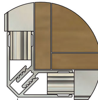
TWO-PIECE ADJUSTABLE CORNER
